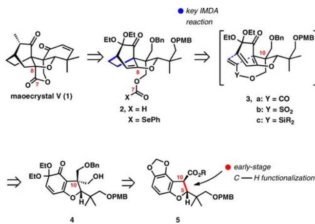
Scheme 1. Synthesis Design for Maoecrystal V
